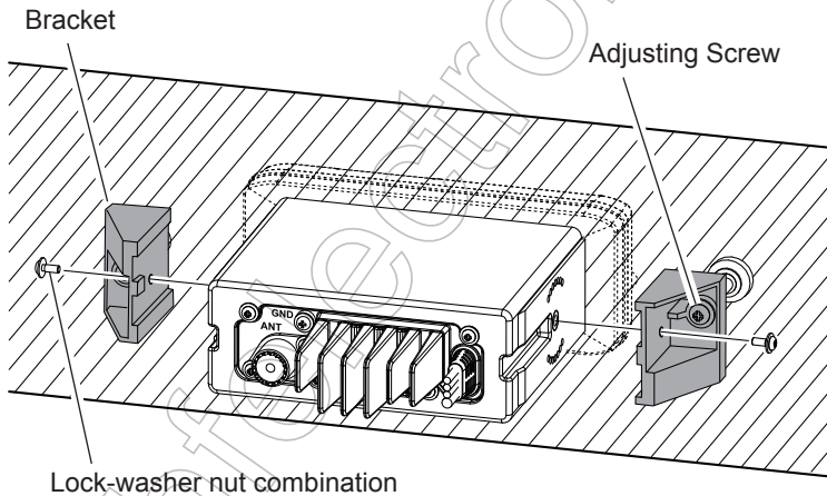
MMB-84 Flush Mount Installation
